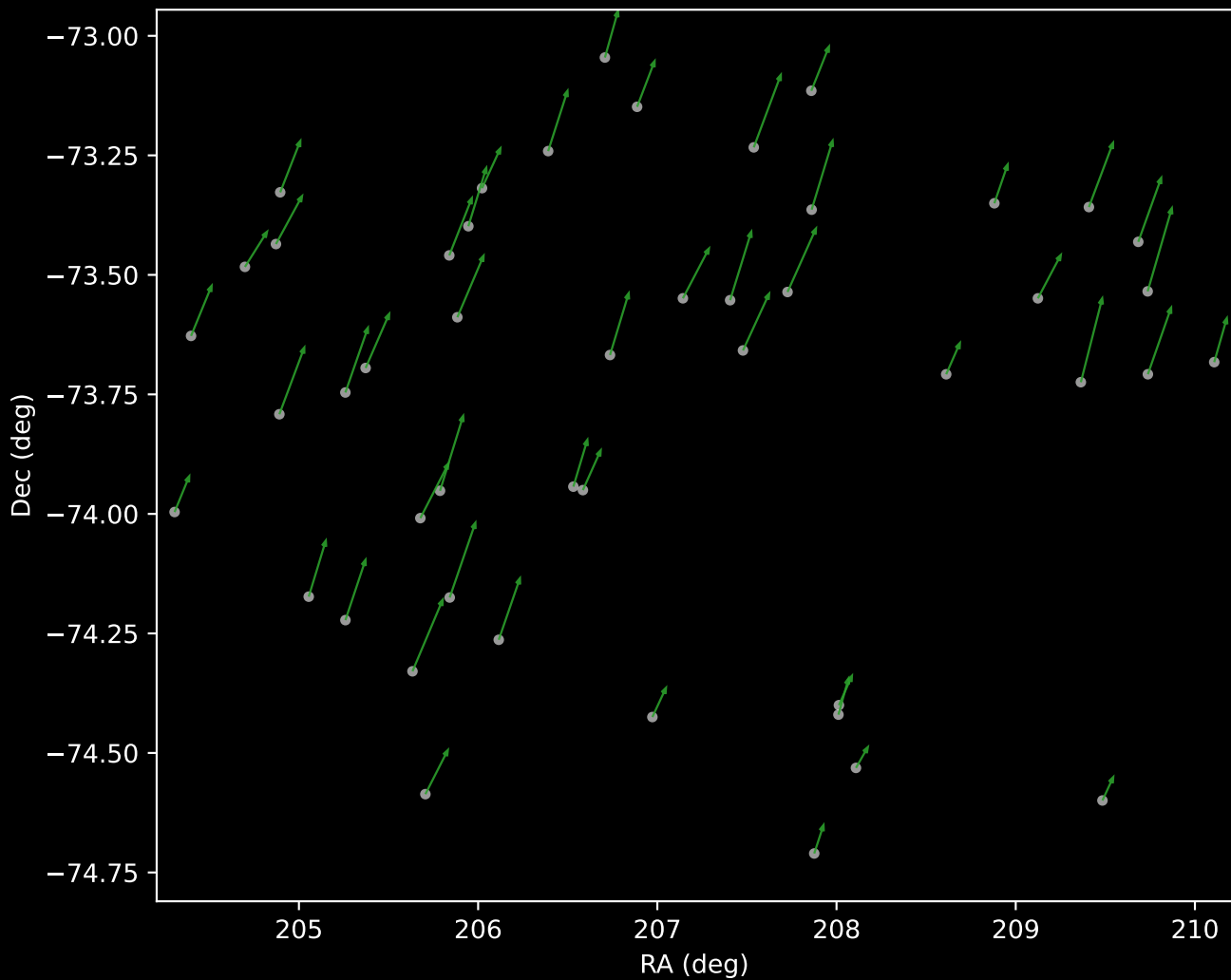
APOGEE DR17 Cluster 4 Proper Motion Vectors (n=48)
