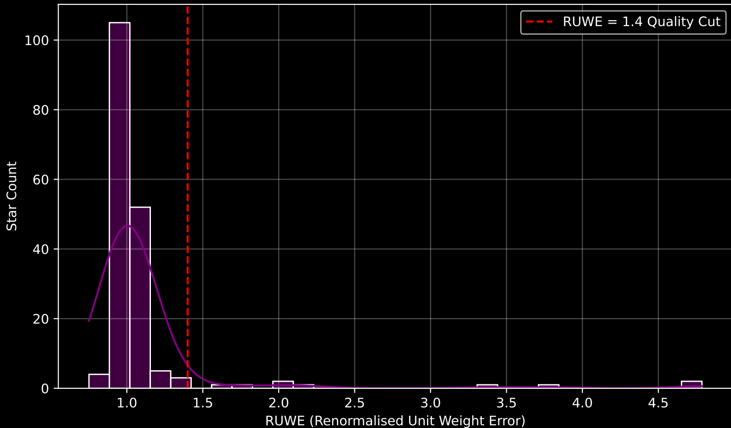
GAPOGEE DR17 Field [LMC23] RUWE Distribution (n= 178)
