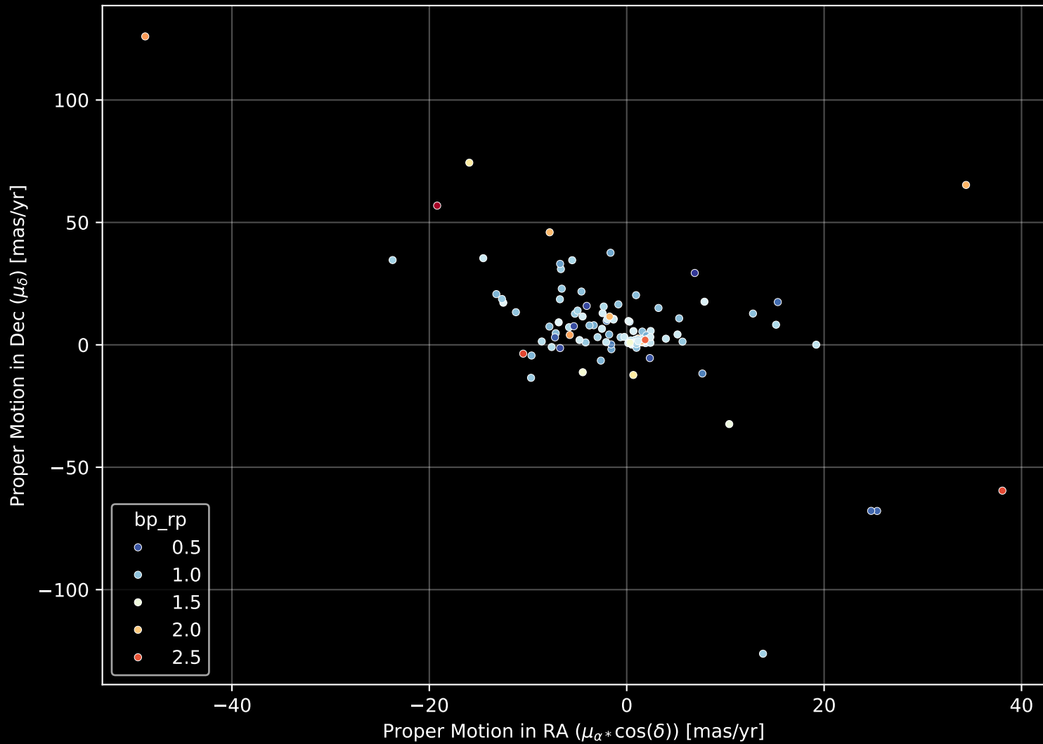
APOGEE DR17 Field: [LMC23] Proper Motion Diagram (n= 178)
