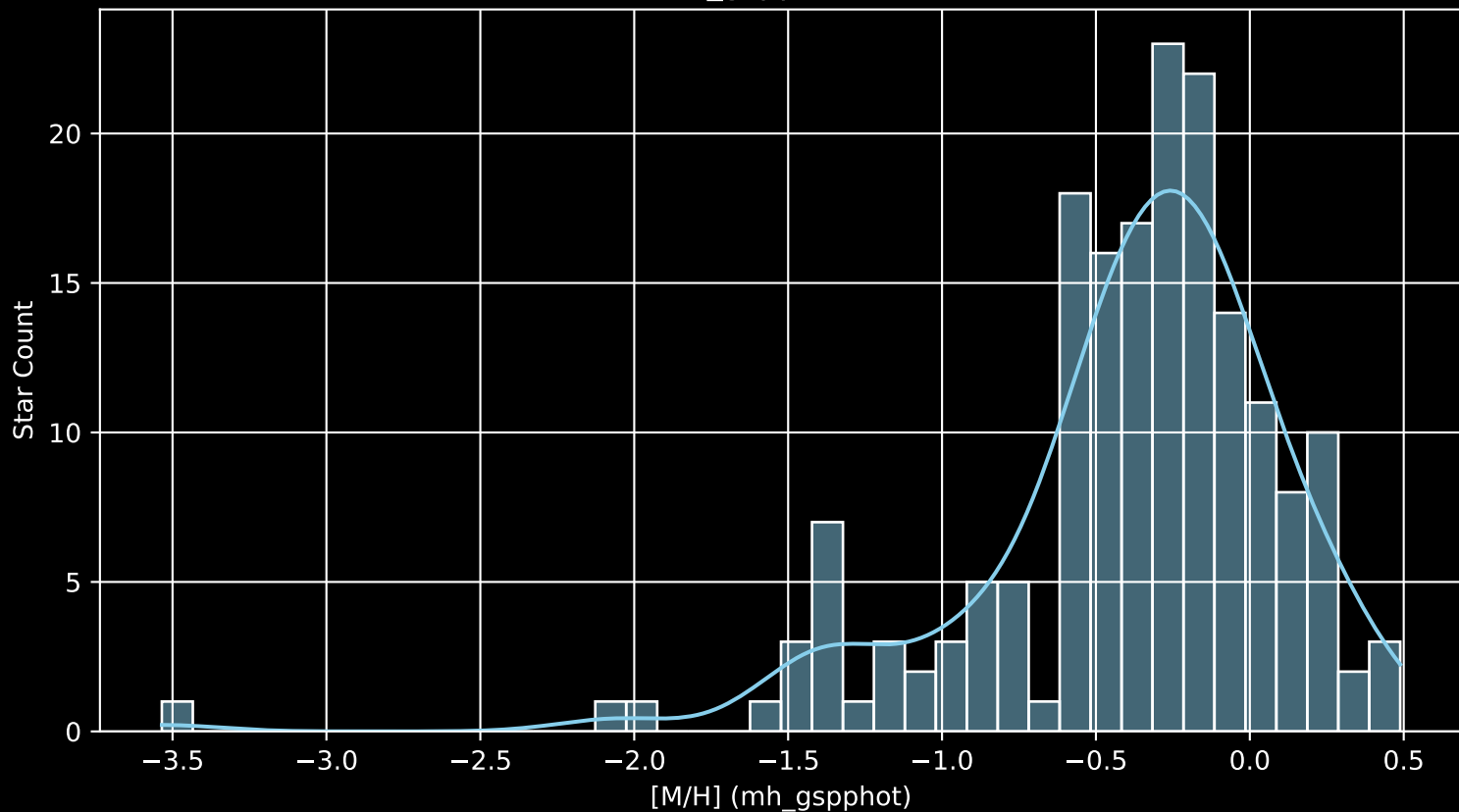
APOGEE DR17 Field: [LMC23 [M/H] (mh_gspphot) (n= 178)
