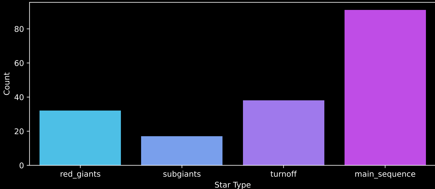
APOGEE DR17 Field: [LMC23] Count plot of Star Type
